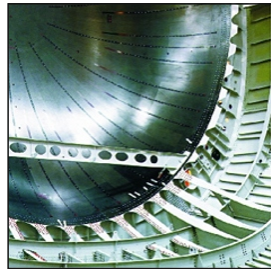
„One Shot Drilling“ CFK/Ti/Al-Stacks
