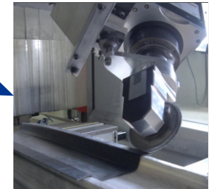
Curved Circular Cutting
