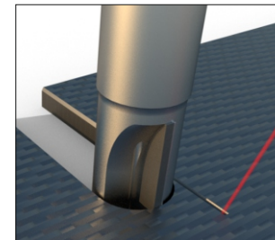
Laser Scored Machining von CFK
